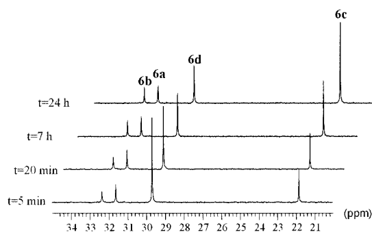
Figure 6. Kinetic 31 P NMR monitoring of crystals of 6 dissolved in CDCl 3
