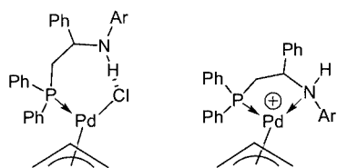
Figure 2. Coordinative features of aminophosphane L 1 in neutral and cationic allyl palladium complexes
